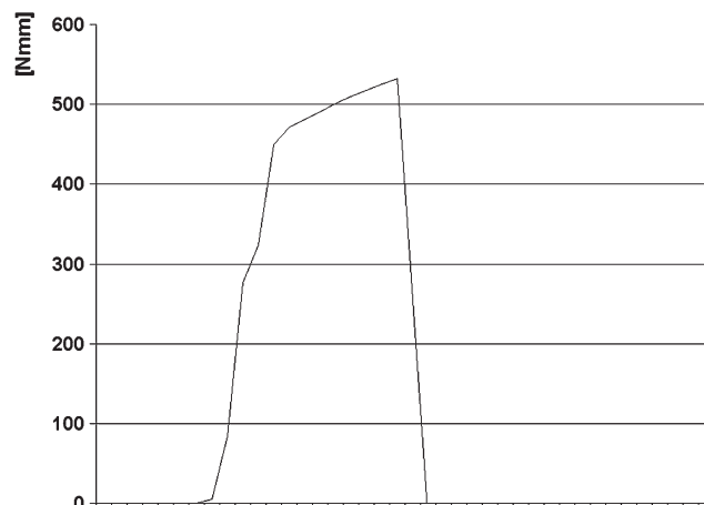
Figure 4 Insertion torque (y-axis) for one mini-implant until fracture (In this case, Bone screw 2 × 10 mm, Stryker). The x-axis represents the insertion procedure.
